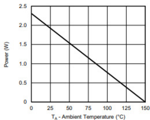
Power, Junction-to-Ambient
