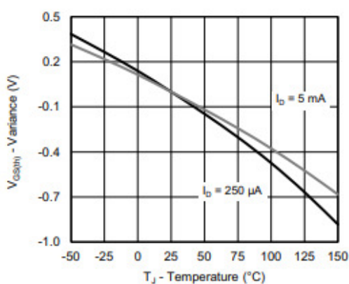
Threshold Voltage
