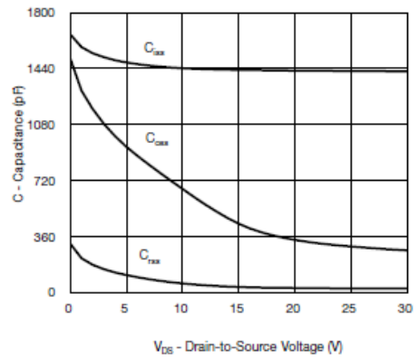
Capacitance
