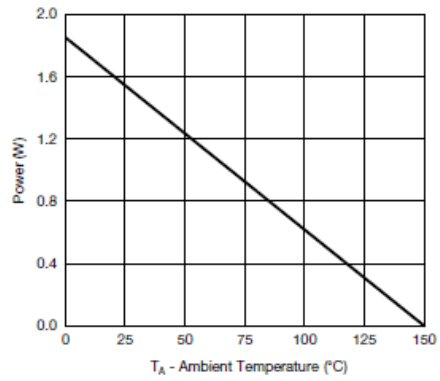
Power, Junction-to-Ambient
