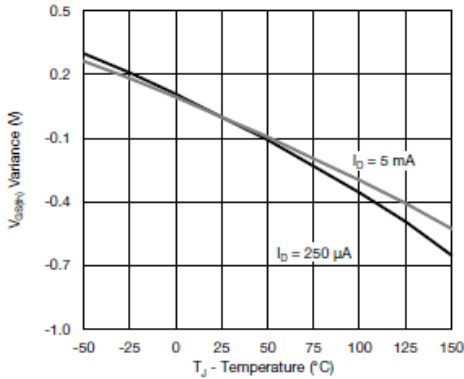
Threshold Voltage
