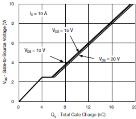
Gate Charge
