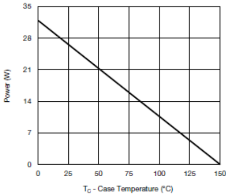
Power, Junction-to-Case
