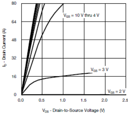
Output Characteristics
