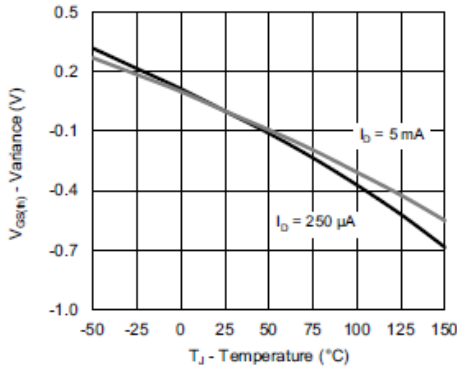
Threshold Voltage
