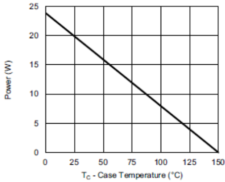
Power, Junction-to-Case
