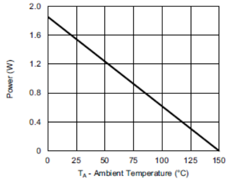
Power, Junction-to-Ambient
