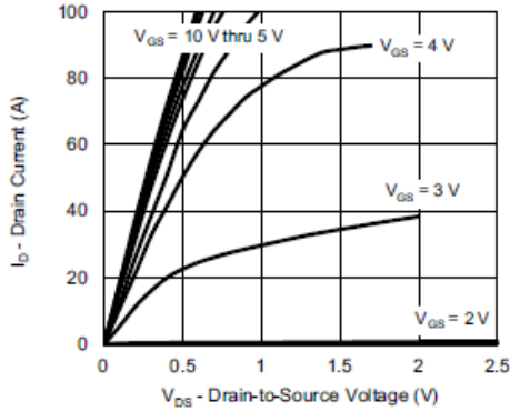
Output Characteristics
