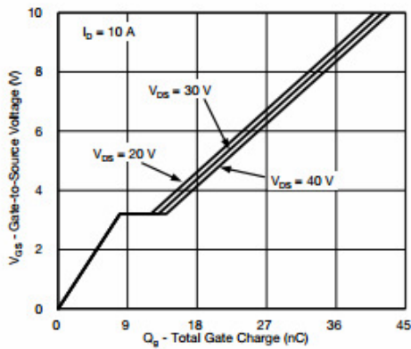
Gate Charge
