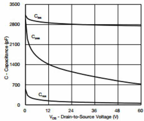
Capacitance
