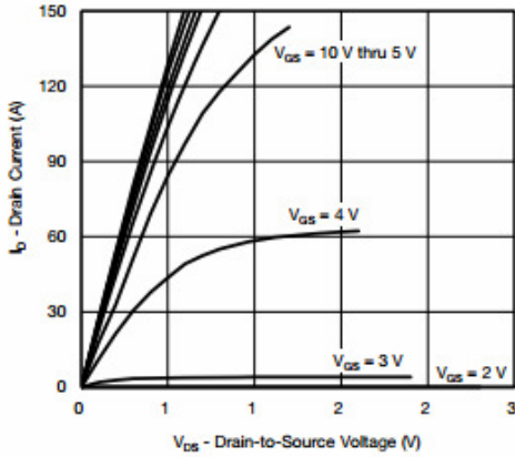
Output Characteristics
