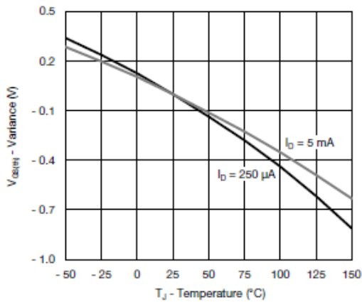
Threshold Voltage
