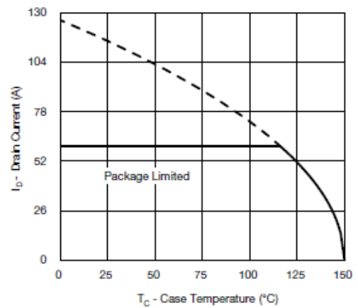
Current Derating*
