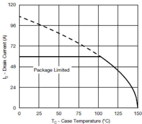
Current Derating*
