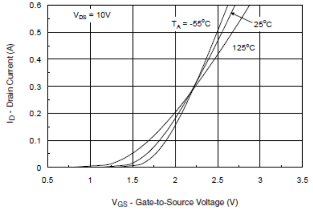
Transfer Characteristics
