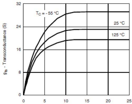
Transconductance
