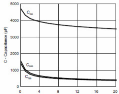
V_{DS} - Drain-to-Source Voltage (V) Capacitance
