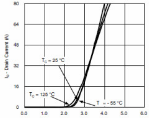
V_{GS} - Gate-to-Source Voltage (V) Transfer Characteristics
