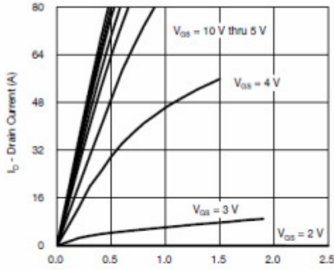
V_{GS} - Drain-to-Source Voltage (V) Output Characteristics
