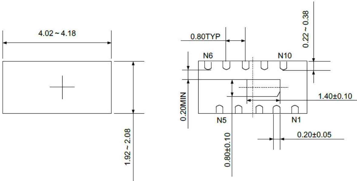
BOTTOM VIEW
